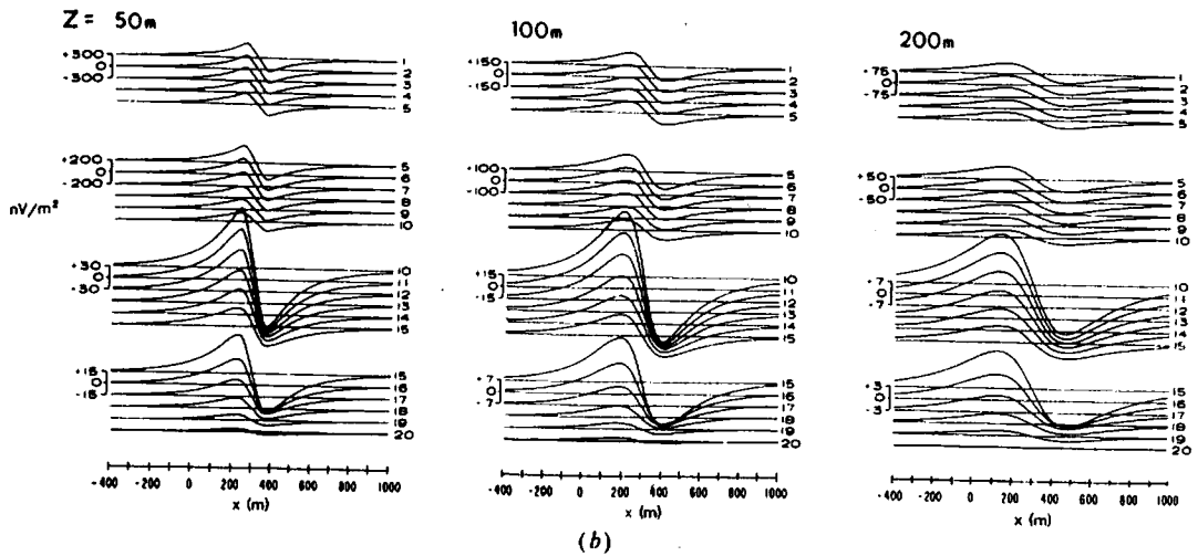
Figure 7.53. (Continued) (b) Variation in \partial H_z/\partial t with depth z ; dip = 90^\circ .
