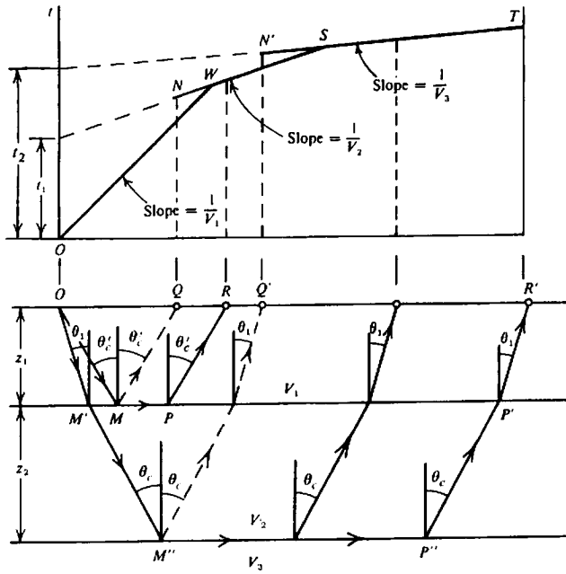
Figure 4.32. Raypaths and traveltimes for the two-refractor case.
