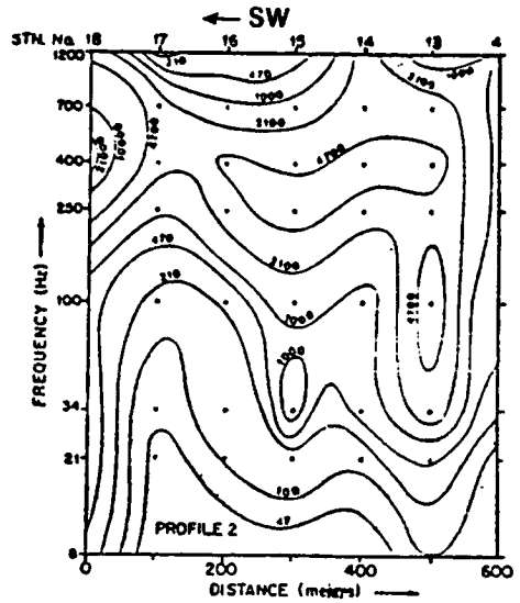
Profile 2 pseudo-section.
