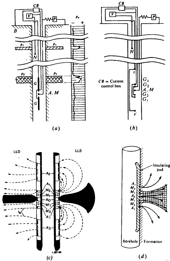
Figure 11.6. Focused current logs. (Courtesy Schlumberger.) (a) Guard log (Laterolog-3). (b) Laterolog-7. (c) Dual laterolog showing how deep and shallow penetration modes of operation can be achieved by reversing the polarity of the A_2 electrodes. (d) Microlaterolog with schematic current flow lines. The shading in (c) and cross-hatching in (d) indicate the current concentration.
