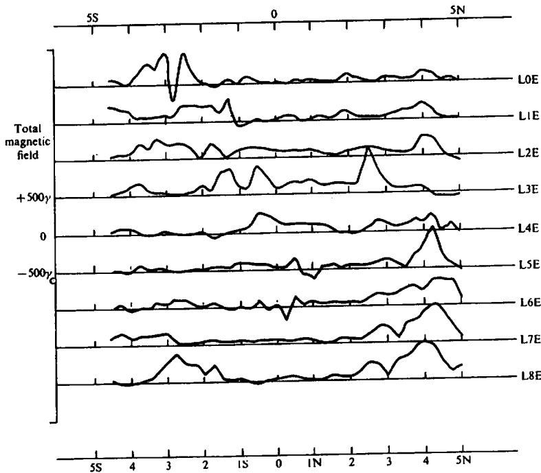
Figure 12.2. Total-field ground-magnetic profiles, Uchi Lake, northwestern Ontario.
