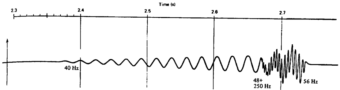
Figure 4.113. Dispersive wavetrain such as that produced by channel waves. The burst of high-frequency energy starting about 2.66 s is superimposed on the low-frequency wave, both ending abruptly at about 2.73 s; this is known as the Airy phase . (From Clay and Medwin, 1977.)
