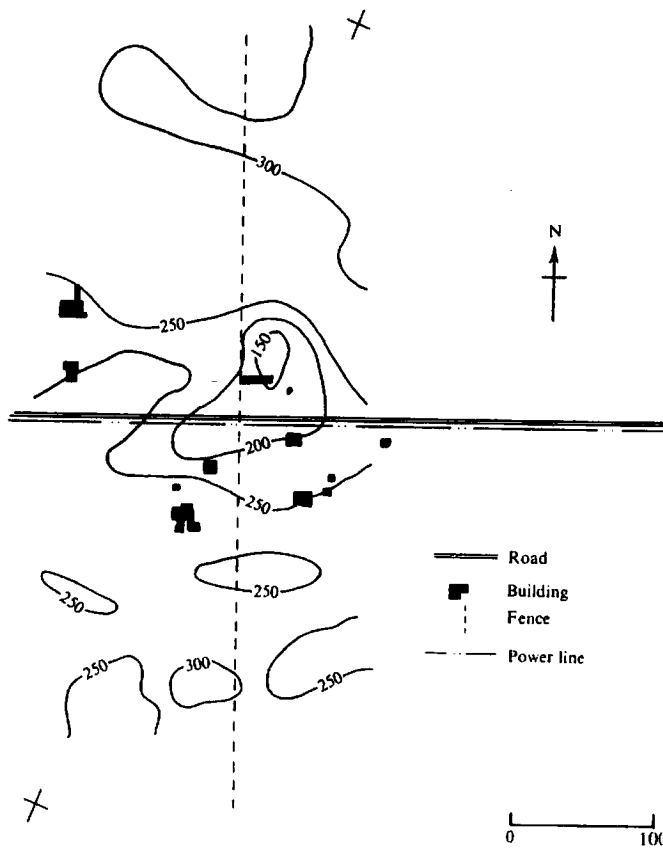
Figure 3.34. Vertical magnetic ground survey, Noranda area; C.I. = 50 nT. (After Seigel, 1957.)
