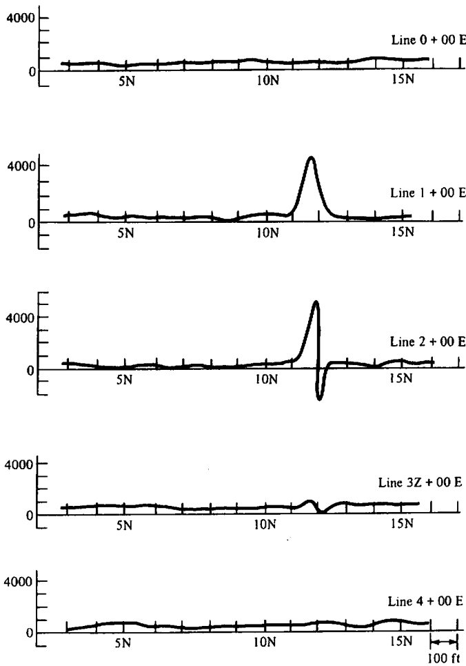
Figure 3.38. Vertical-component magnetic profiles, Rouyn-Noranda district, Quebec.
