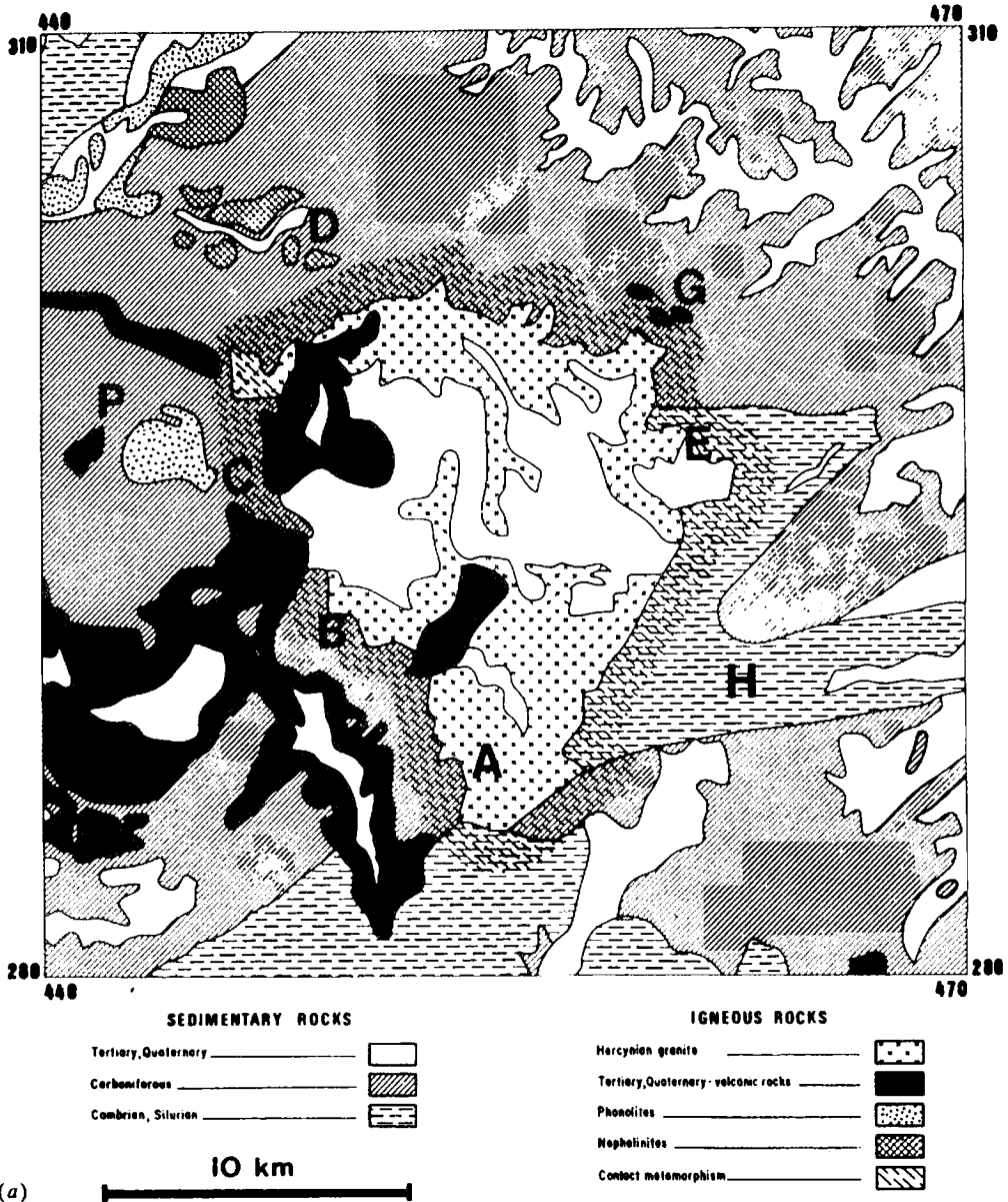
Figure 10.20. Airborne radiometric and magnetic surveys over granite zone, Morocco. (a) Detailed geology of the area.
