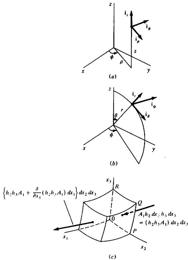
Figure A.4. Curvilinear coordinates. (a) Cylindrical coordinates. (b) Spherical coordinates. (c) \text{div} \mathbf{A} in curvilinear coordinates.
