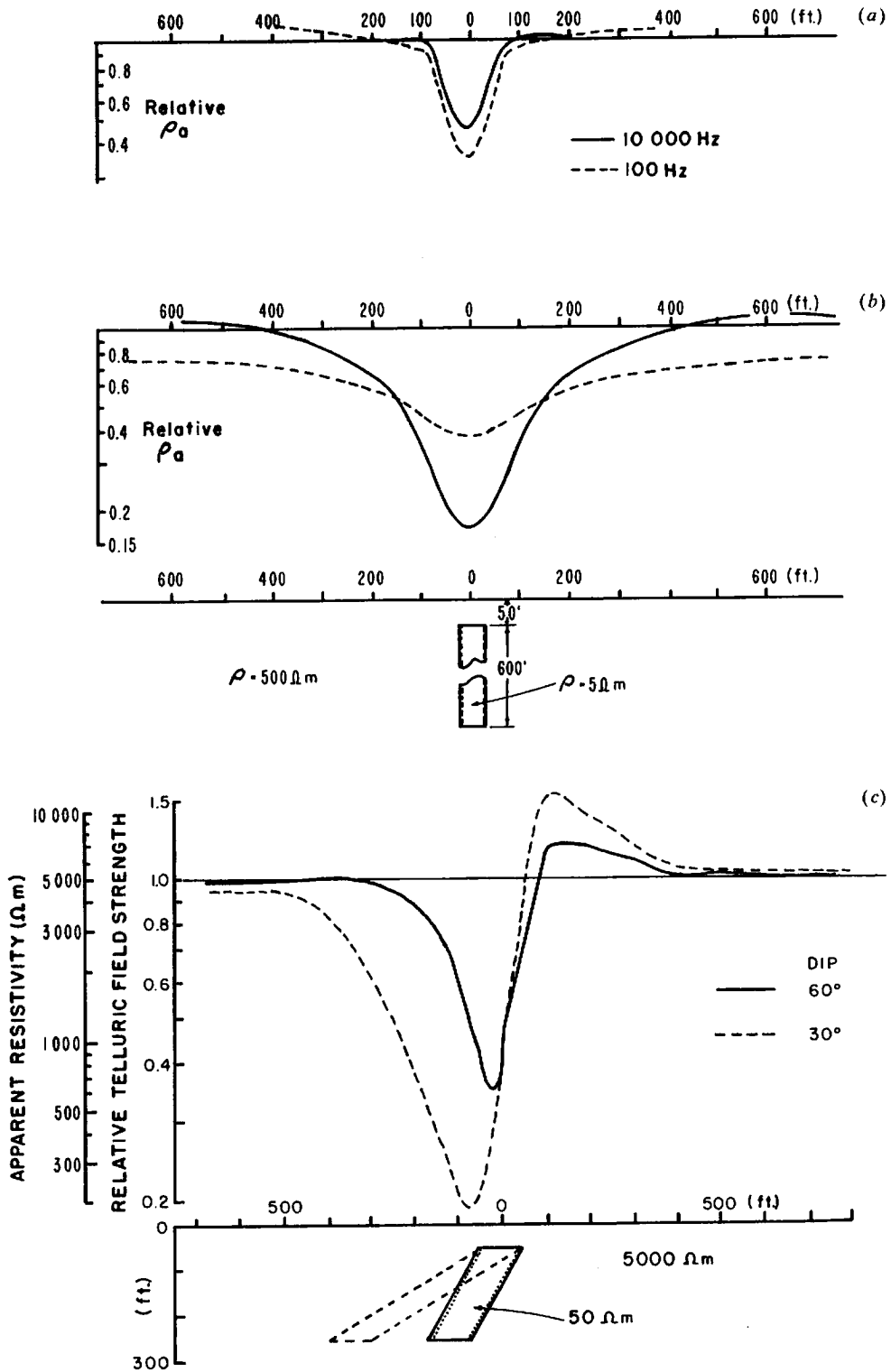
Figure 6.19. Theoretical resistivity profiles over vertical dike [(a) and (b)] and dipping dike (c). (a) E_{\perp} polarization. (b) E_{\parallel} polarization. (c) E_{\perp} polarization.
