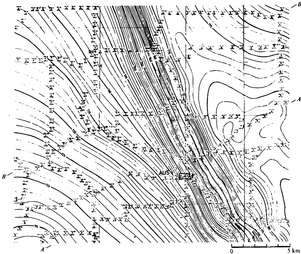
Figure 2.46. Bouguer gravity map, Western Australia; C.I. = 1.0 \text{ mGal} . (Courtesy West Australian Petroleum.)
