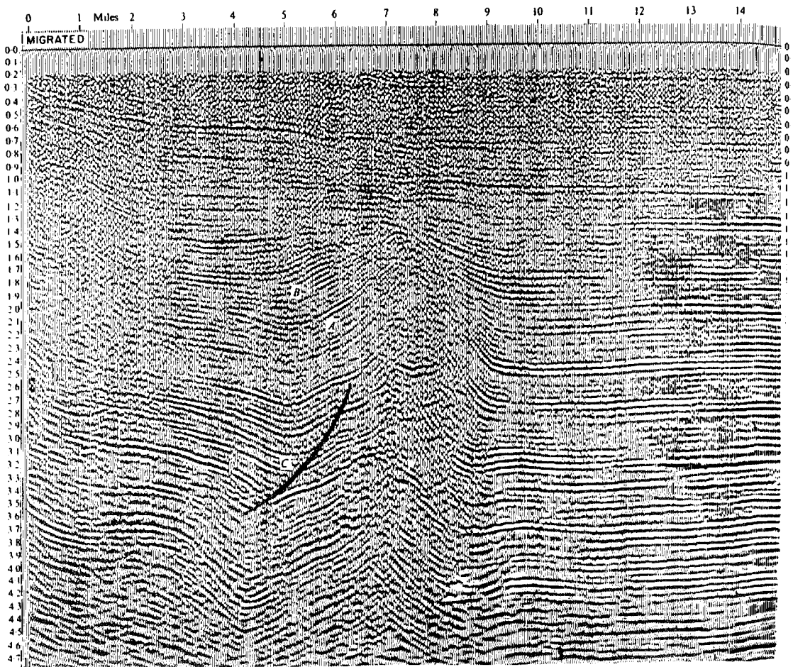
Figure 4.101. Migrated section across a faulted anticline in the San Joaquin Valley of California. The main anticline is associated with a nearly vertical reverse fault. (Courtesy Texaco.)
