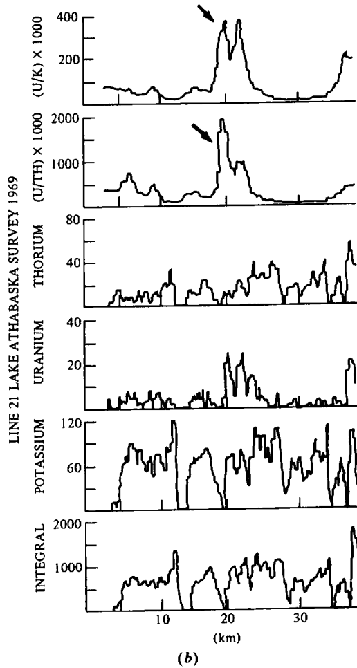
Figure 10.10. Airborne \gamma -ray spectrometer profiles. (a) Total-count profiles in the Elliot Lake and Bancroft areas, Ontario. (b) Four-channel results, Uranium City area, Saskatchewan. (After Darnley, 1970.)
