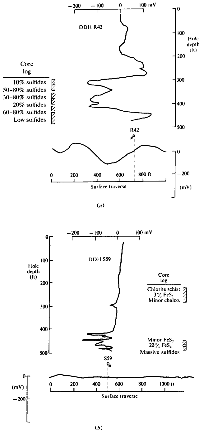
Figure 6.7. Surface and drill-hole SP for different overburdens. (a) Sand overburden. (b) Clay overburden.
