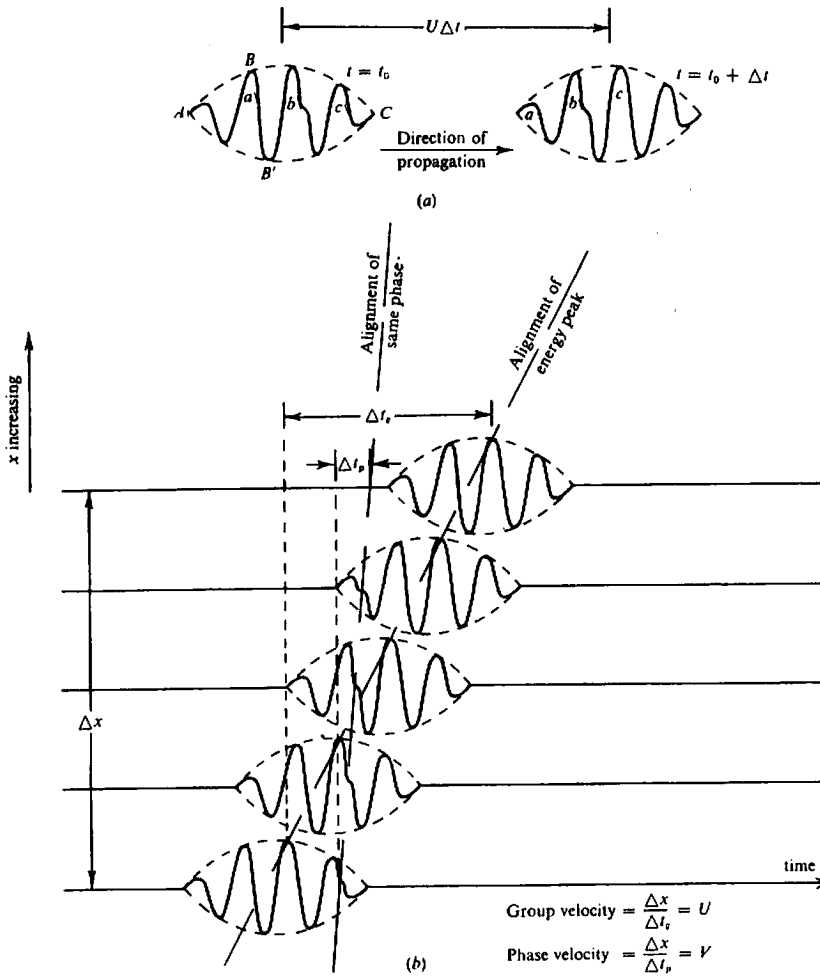
Figure 4.14. Comparison of group and phase velocities. (a) Definition of group velocity U . (b) Arrival of a dispersive wave at successive geophones.
