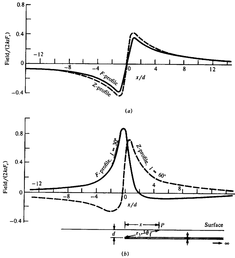
Figure 3.22. Semiinfinite horizontal sheet. F , Z profiles for (a) N-S strike, I = 60°; (b) E-W strike, I = 60 and 30°.
