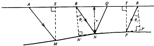
Figure 4.88. Determining sourcepoint and geophone delay times.
