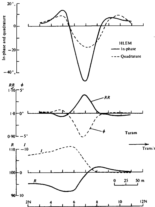
Figure 7.115. HLEM and Turam profiles, northern Quebec.
