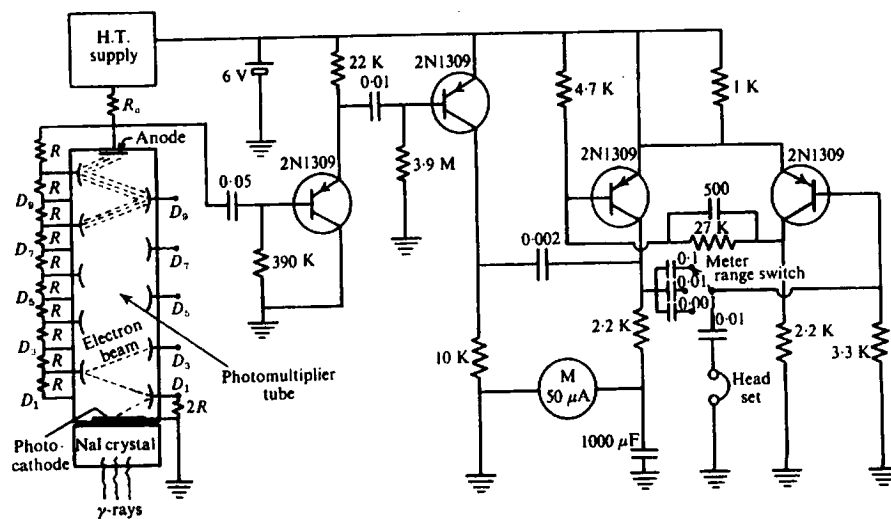
Figure 10.5. Scintillation-meter schematic.
