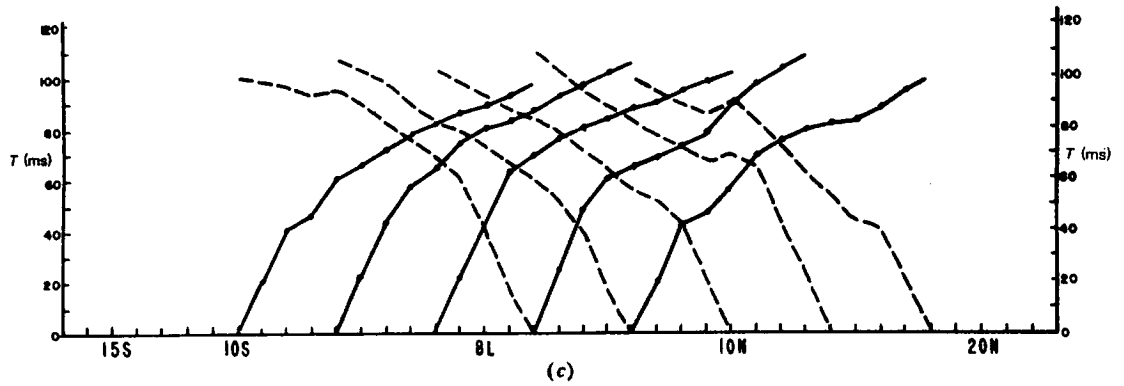
Figure 12.17. (Continued) (b) Typical reversed refraction profiles, line 16E. (c) Refraction time-distance plot, line 16E.
