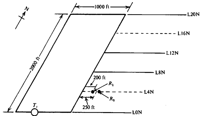
Figure 7.114. Model Turam configuration.
