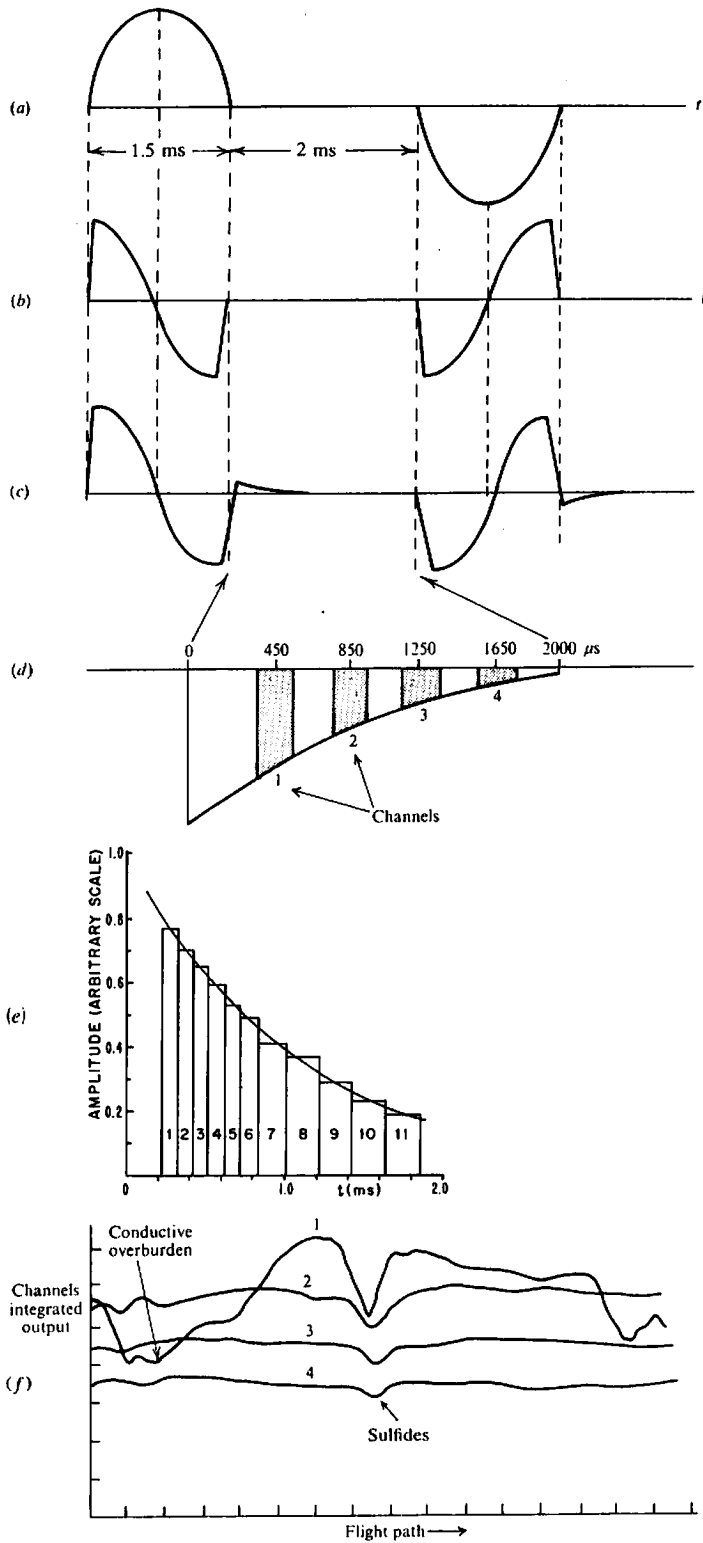
Figure 7.28. Input airborne EM system. (a) Primary magnetic field, H_p . (b) Receiver-coil voltage due to H_p when H_z = 0 . (c) Receiver-coil voltage due to H_p + H_s . (d) Decay signals in the four sampling channels. (e) 11-channel sampling with zero off-time between. (f) Four-channel record over Texas Gulf Sulphur, Timmins, Ontario.
