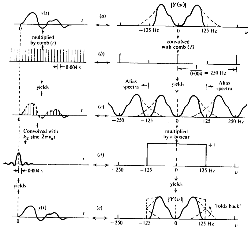
Figure 4.78. Sampling and reconstituting.
