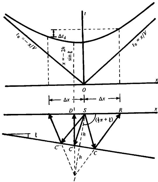
Figure 4.23. Geometry and traveltime curve for dipping reflector.
