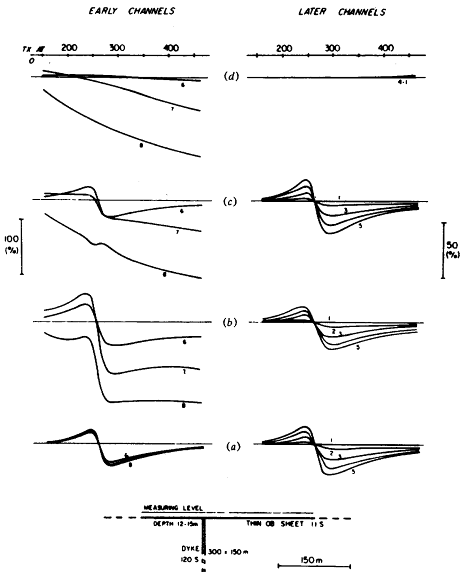
Figure 7.63. Model UTEM H_2^2 profiles over a vertical conductive sheet under a thin conductive overburden. (After West, Macnae, and Lamontagne, 1984.) (a) Effect of sheet alone. (b) Sheet in contact with the overburden. (c) Sheet not in contact with overburden. (d) Overburden alone.
