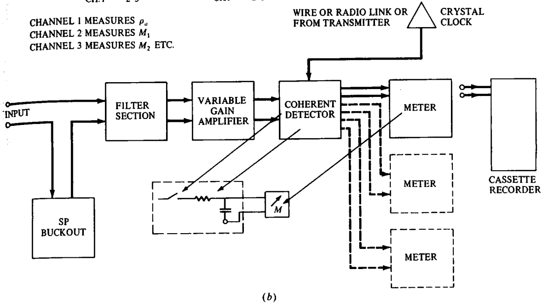
Figure 9.6. (Continued) (b) F-D receiver. (After Sumner, 1976.)
