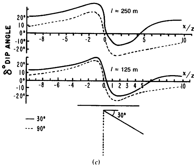
Figure 7.30. Response of dip-angle fixed-transmitter system to dipping sheets. l = T-R . (After Ward, 1967.) (a) Sheets of depth extent d dipping 30 and 60°. (b) Effect of variable depth of vertical sheet. (c) Effect of T-R separation.
