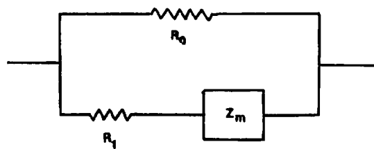
Figure 9.3. Equivalent electrical circuit to simulate the IP effect.
