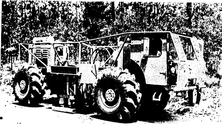
Figure 4.52. Vibrators mounted for off-road survey. (Courtesy Conoco.)
