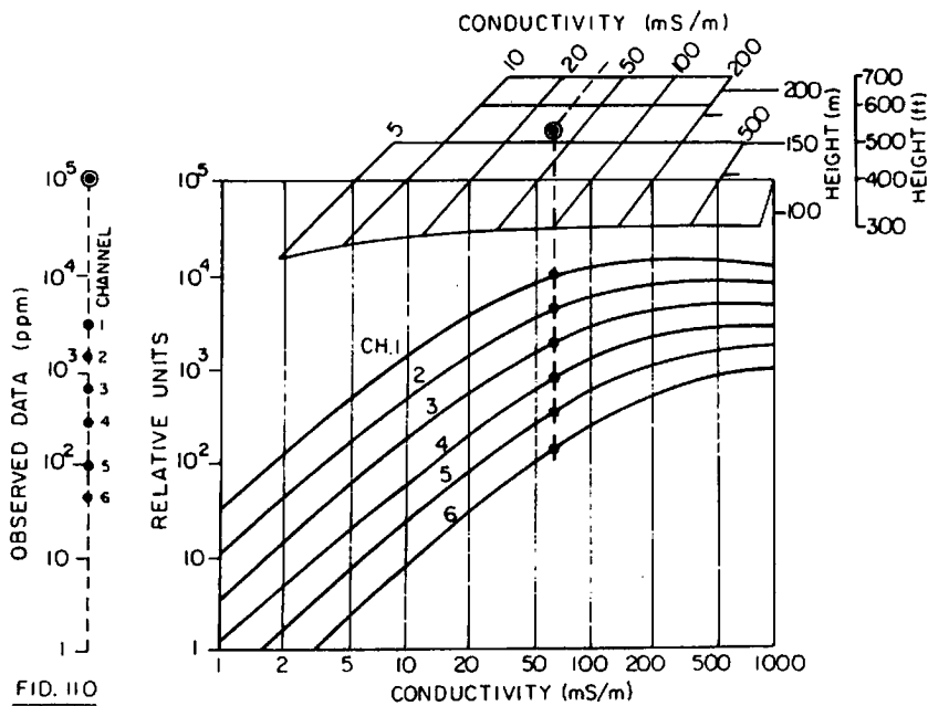
Figure 7.88. (Continued) (b) Palacky nomogram for interpreting conductivity and aircraft height (above the conductor) for a conductive half-space. (After De Mouly and Becker, 1984.)
