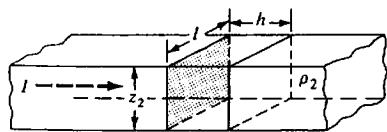
Figure 8.31. The equivalence principle (schematic). (a) \rho_1 < \rho_2 > \rho_3 , \rho_2 z_2 = \text{constant} . (b) \rho_1 > \rho_2 < \rho_3 , \rho_2 / z_2 = \text{constant} .
