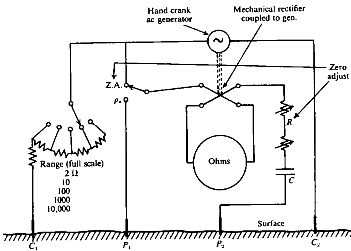
Figure 8.17. Portable equipment for measuring resistivity (schematic).
