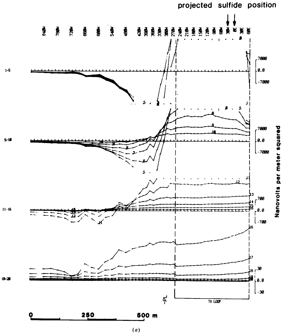
Figure 7.103. EM37 profiles, line 100S. White Leads prospect, Broken Hill, New South Wales. (After Smith, 1985.) (a) Vertical components.
