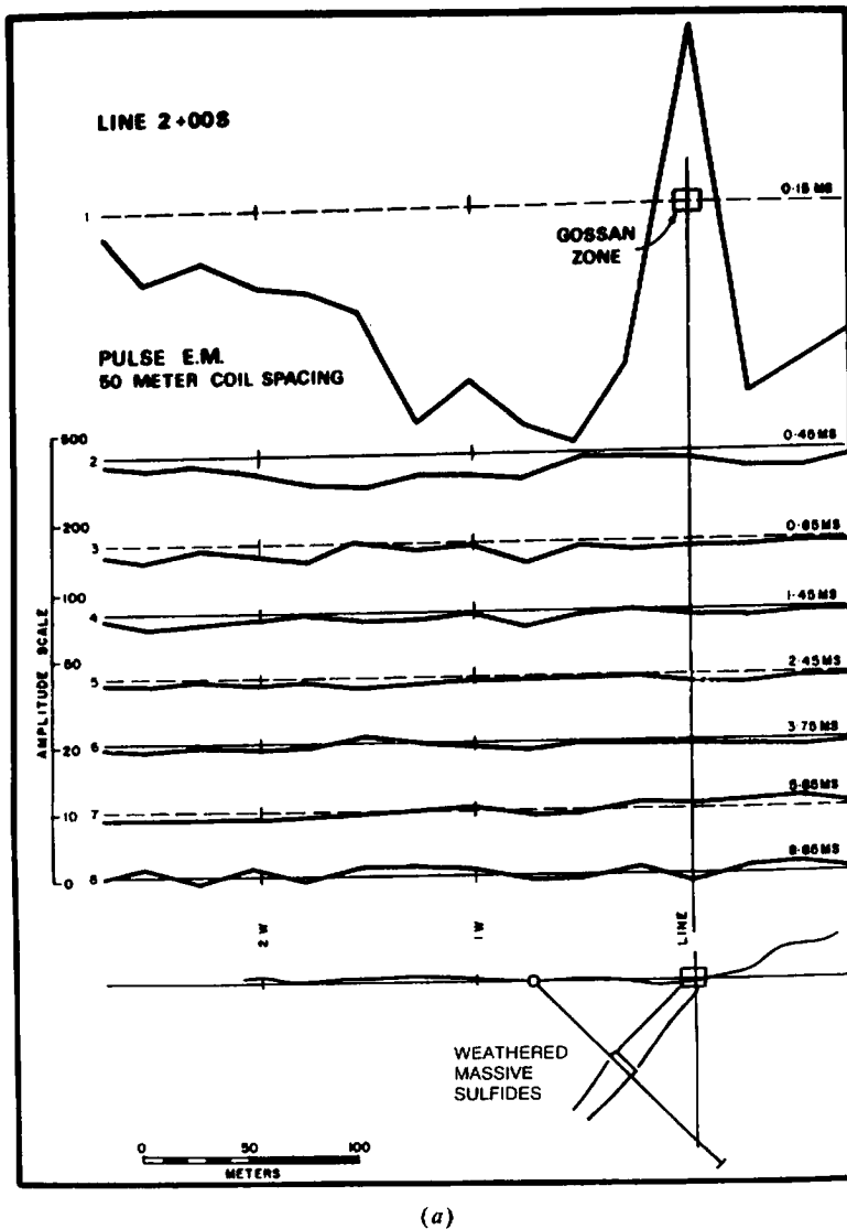
Figure 7.101. Results of PEM base-metal survey in Sultanate of Oman using moving-coil method and interpretation using a model plate. [Parts (a) and (b): After Crone, 1979; parts (c) and (d): After Bartel and Hohmann, 1985.] (a) Profile over Ghayth showing: 50 m coil spacing.
