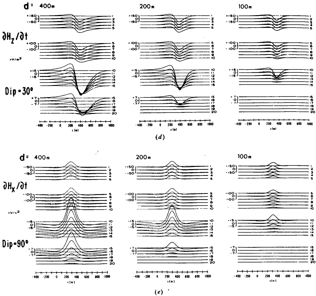
Figure 7.53. (Continued) (d) Effect of depth extent d on \partial H_z/\partial t , z = 100 m, \ell = 800 m, dip = 30^\circ . (e) Same as (d) except for H_x and dip = 90^\circ .
