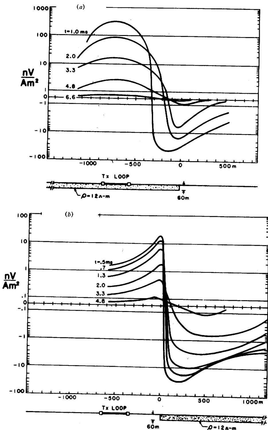
Figure 7.54. Comparison of responses of Turam-type (TDEM) and SIROTEM(1) over conductive overburden. Turam: Tx loop 600 x 300 m in (a), (b), and (c). (After Spies and Parker, 1984.) (a) Tx on overburden ~ 550 m from edge. (b) Tx offset ~ 350 m from edge.
