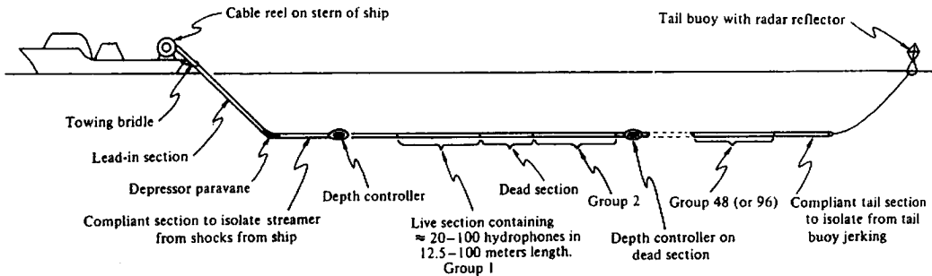
Figure 4.64. Streamer. (After Sheriff, 1984.)
