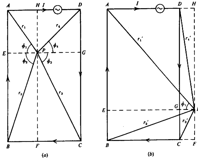
Figure 7.2. Geometrical parameters involved in calculating the magnetic field of a rectangular loop. (a) Calculating the field at an internal point; (b) Calculating the field at an external point.
