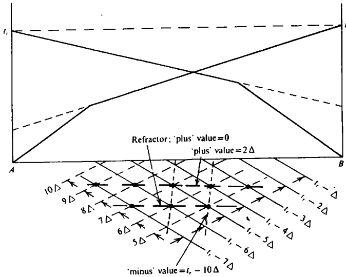
Figure 4.94. The plus-minus method. (After Hagedoorn, 1959.)
