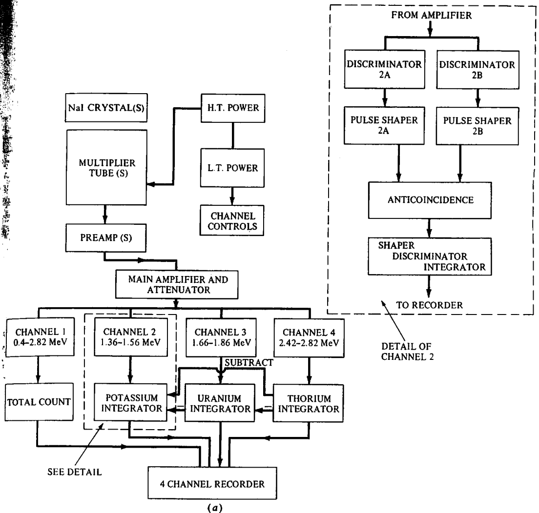
Figure 10.8. Four-channel \gamma -ray spectrometer. (a) Block diagram.
