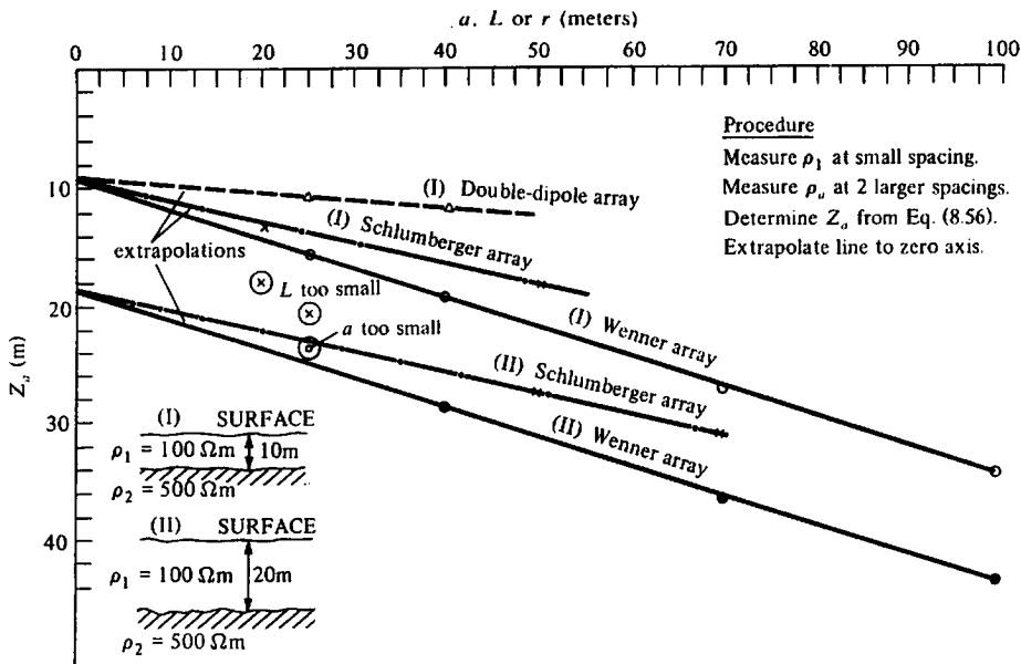
Figure 8.39. Graphical determination of overburden thickness using one small spread to get \rho_1 and two large spreads to get z_a .
