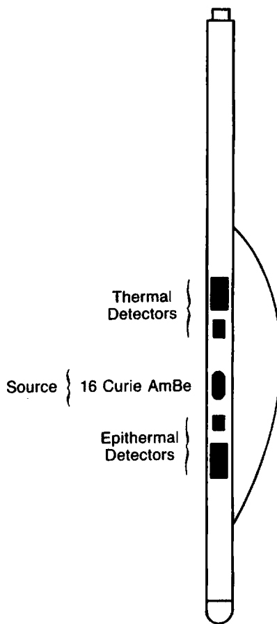
Figure 11.38. Schematic of dual-porosity neutron-logging sonde. (From Schlumberger, 1987.)
