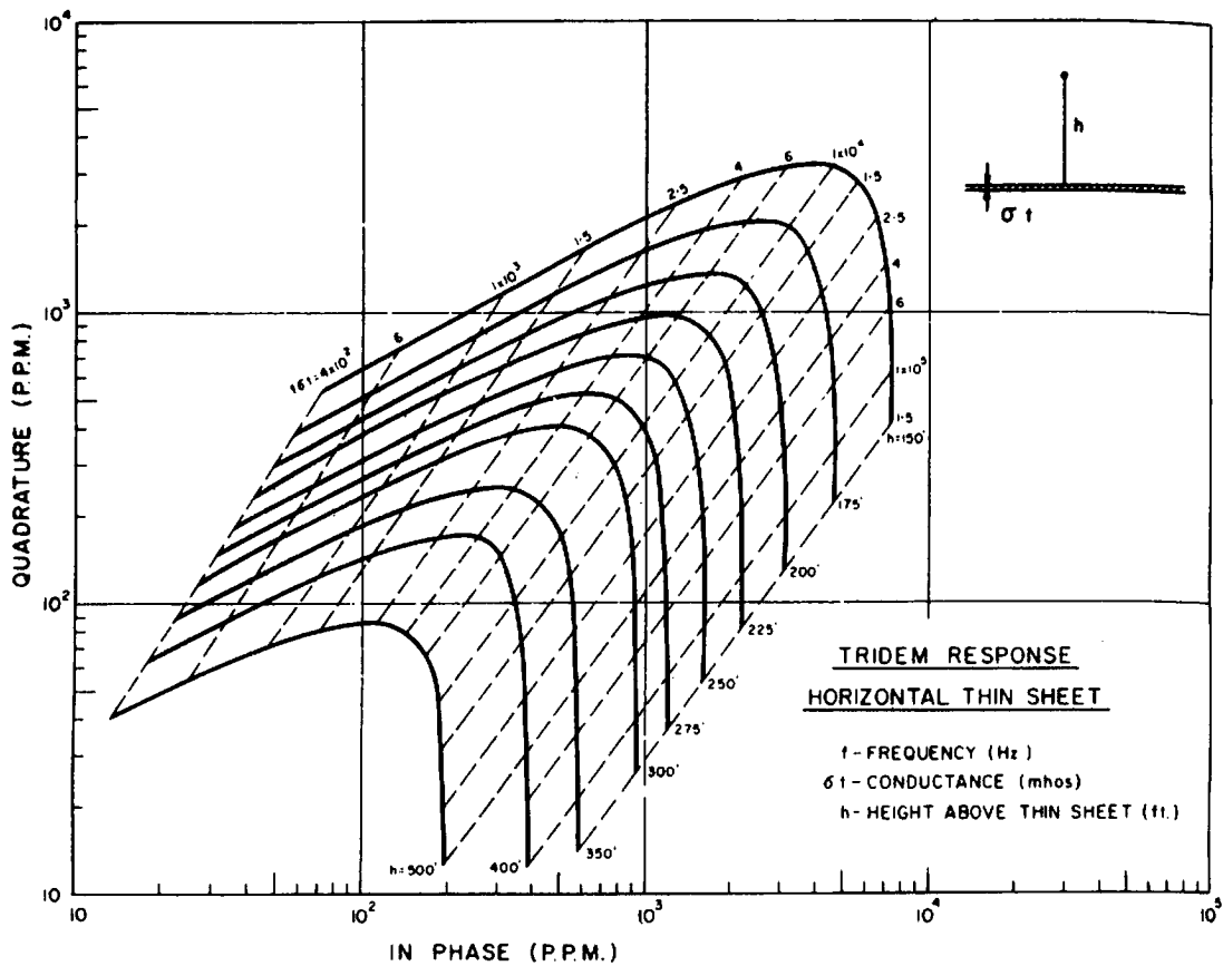
Figure 7.83. Characteristic curves for the Tridem system over a horizontal thin sheet. Solid-line curves are for constant ( ft ), dashed are for constant h .
