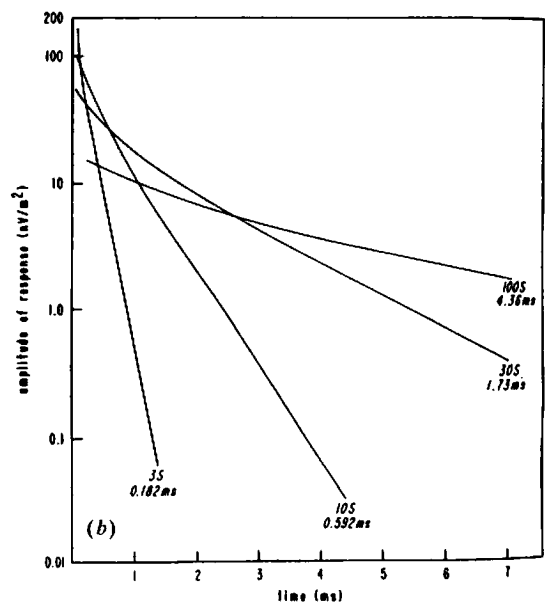
Figure 7.67. Nomograms for estimating at product. (a) PEM(1) system, channel ratios versus TCP (numbers at ends of curves denote channels); model plate 600 \times 600 m, z = 50 m, dip = 30^\circ , T - R = 100 m. (After Bartel and Hohmann, 1985.) (b) EM37 system, curves of response amplitude versus time for various values of TCP (or time constant); model plate 800 \times 400 m, z = 50 m, dip = 90^\circ . (After Gallagher, Ward, and Hohmann, 1985.)
