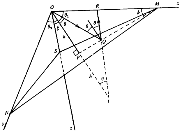
Figure 4.26. Three-dimensional view of a reflection path for a dipping bed.
