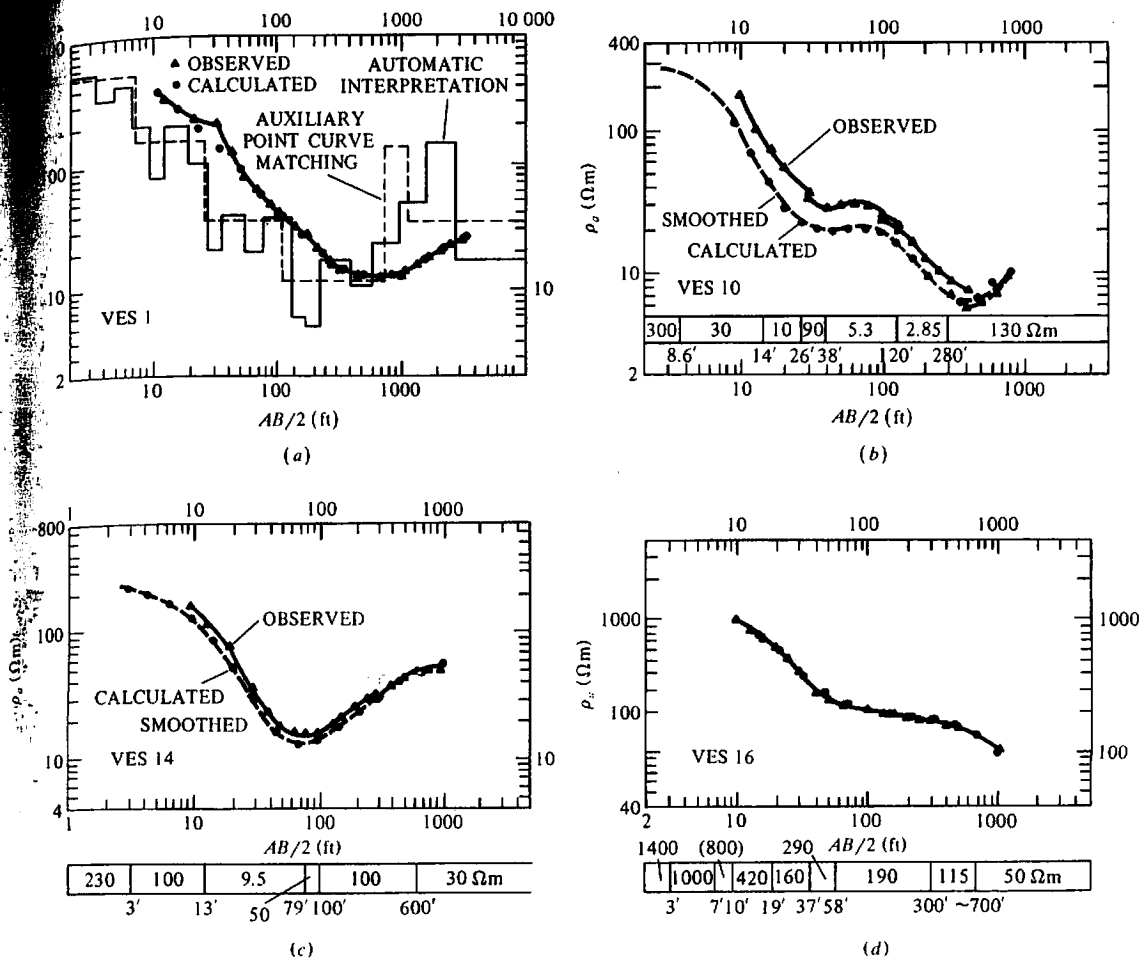
Figure 8.44. Soundings used to obtain geoelectric section in Figure 8.43. ▲ and ○ denote observed and calculated values. (Note the alternative plotting methods used in (a) and (b); see also Figs. 8.29 and 8.42.) (After Zhody, Anderson, and Muffler, 1973.) (a) VES 1 interpreted by partial curve matching (6-layer) and complete curve matching (19-layer). (b) VES 10, partial curve matching (7-layer). (c) VES 14, partial curve matching (6-layer). (d) VES 16, complete curve matching (9-layer).
