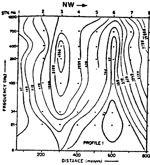
Profile 1 pseudo-section.
