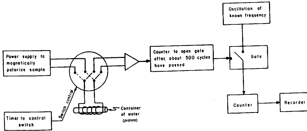
Figure 3.10. Proton-precession magnetometer. (From Sheriff, 1984.)
