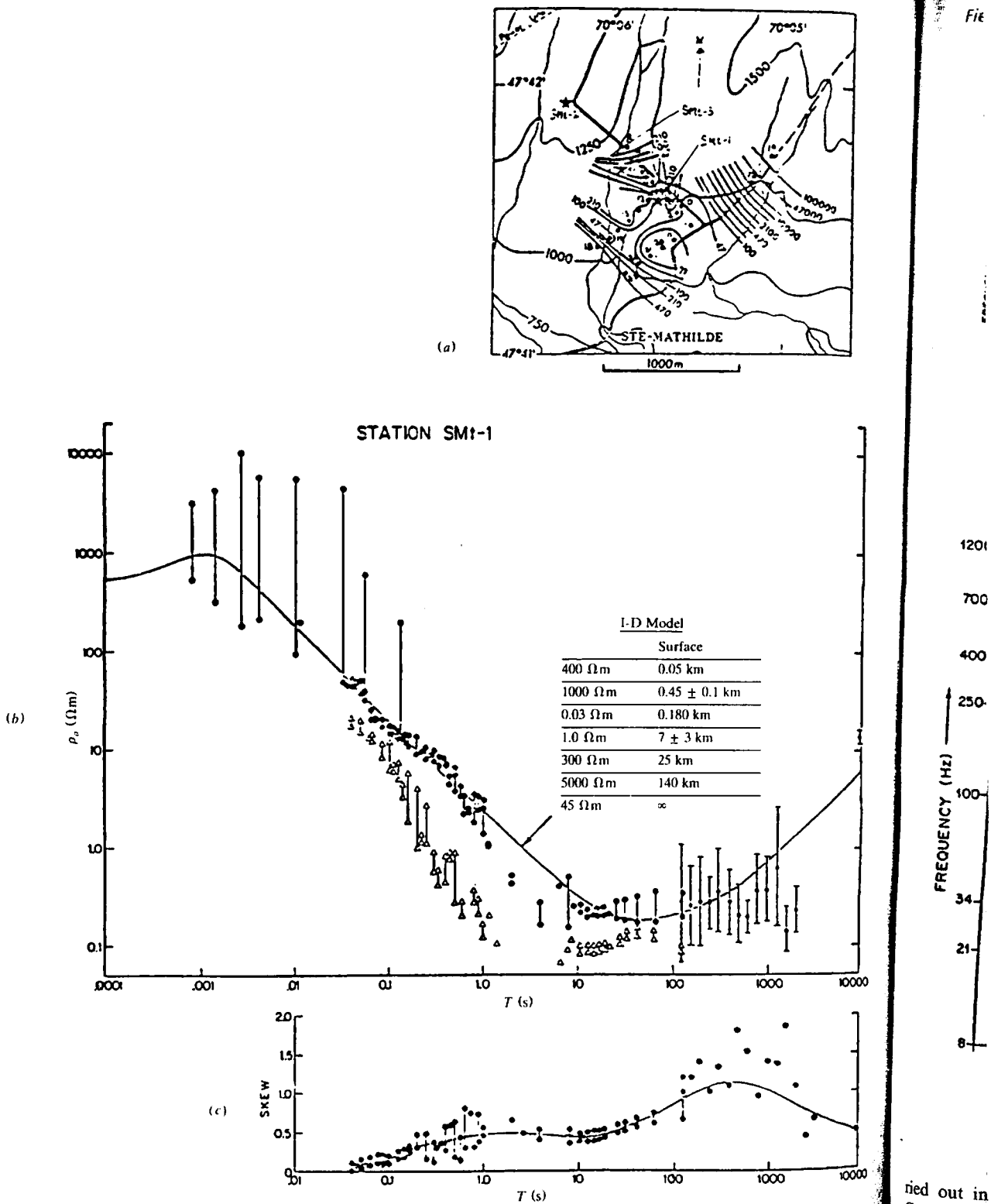
Figure 6.30. \rho_a results near Ste. Mathilde, Quebec. (a) Map showing elevations, locations of profiles 1 - 3 plus \rho_a contours. (b) Results for station SM1-1: \rho_a curve, tensor data in the principal axis of anisotropy from 0.03 to 10,000 s, and scalar data from 0.0008 to 0.13 s; dots and triangles are \rho_a values for the major and minor axes of anisotropy, respectively; error bars show maximum scatter from 0.0008 to 100 s, two standard deviations from 100 to 10,000 s; solid curve is for the 1-D model. (c) Skew ratios.
