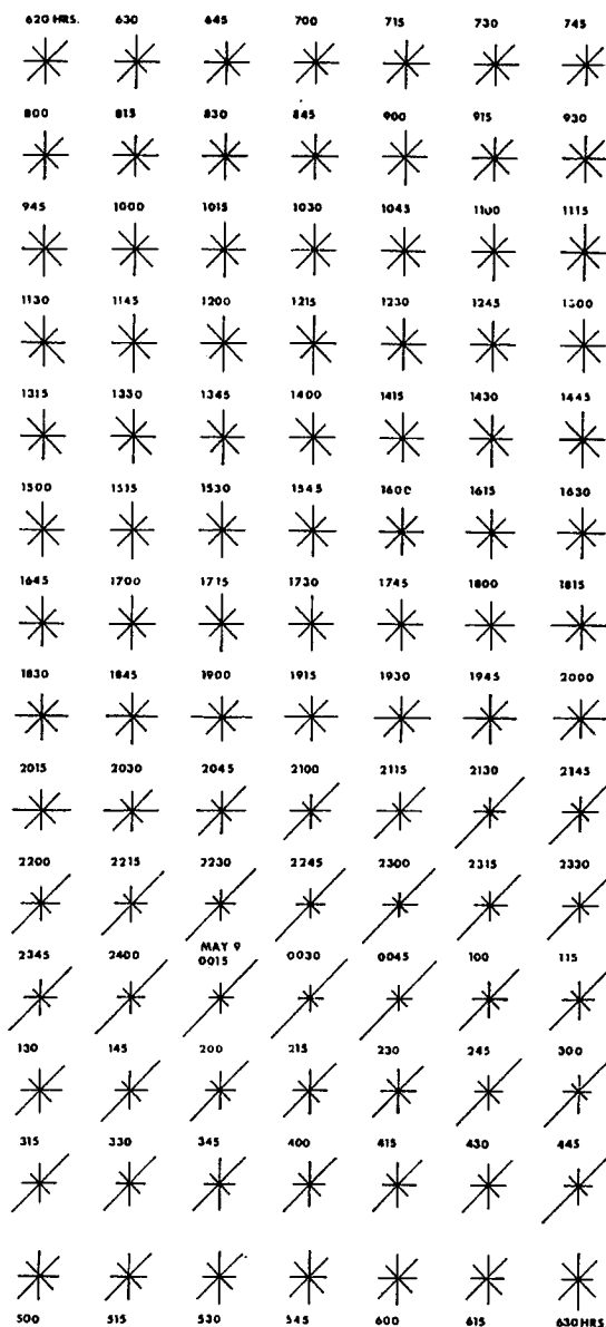
Figure 6.12. Anisotropic telluric response, Vale Perkins, Quebec, May 8-9, 1975. Frequency 145 Hz.
