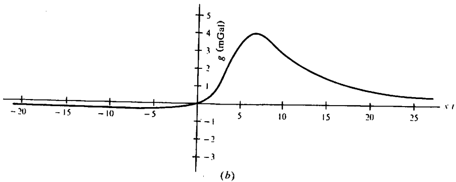
Figure 2.29. Gravity effect of a faulted horizontal sheet; t = 300 m, h_1 = 750 m, h_2 = 1350 m, and \rho = 1 g/cm 3 . (a) Normal fault dipping \alpha = 30 and 90^\circ . (b) Reverse fault, \alpha = -30^\circ .
