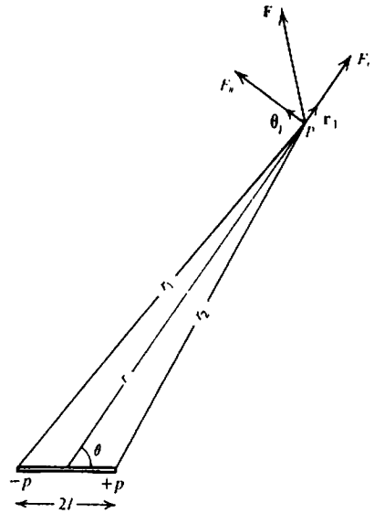
Figure 3.3. Calculating the field of a magnetic dipole.
