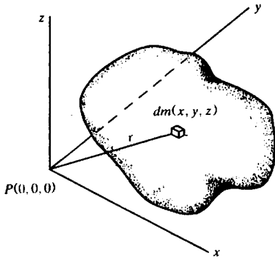
Figure 2.1. Potential of three-dimensional mass.
