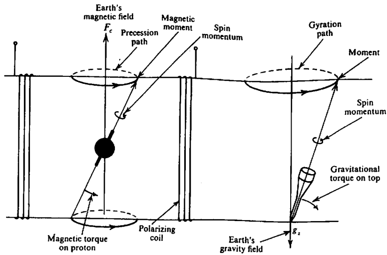
Figure 3.9. Proton precession and spinning-top analogy.
