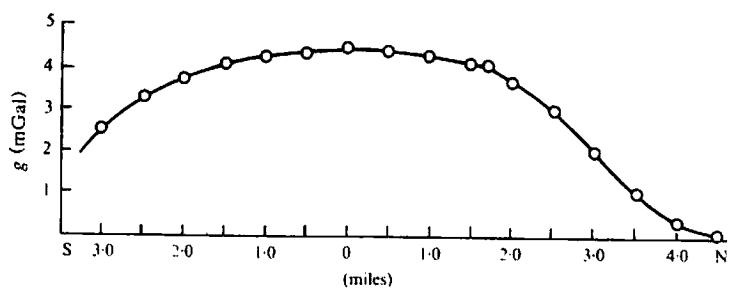
Figure 2.45. Residual gravity profile over three-dimensional structure, St. Lawrence lowlands.
