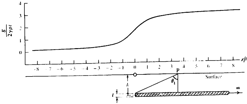
Figure 2.28. Gravity effect of a semiinfinite horizontal sheet.
