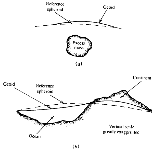
Figure 2.2. Comparison of reference spheroid and geoid. (a) Warping of the geoid by a local mass. (b) Large-scale warping.
