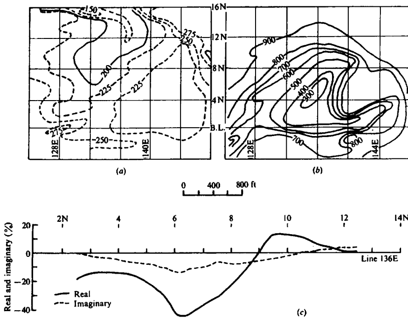
Figure 12.6. Magnetic and electrical data, Murray sulfide deposit, New Brunswick. (a) Magnetic contours; contour interval 25 \gamma . (b) SP contours; contour interval 100 mV. (c) HLEM profile; frequency 440 Hz, T-R spacing 300 ft.
