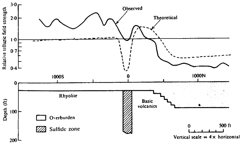
Figure 12.4. Telluric profile and geologic section, Mobern Sulphide Deposit, northwestern Quebec. For theoretical model, \rho_{sul} = 1 \Omega m , \rho_{over} = 70 \Omega m , and \rho_{host} = 7,000 \Omega m .
