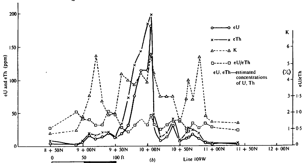
Figure 10.19. Results of radiometric survey over pegmatite, Portneuf, Quebec. (a) Isorad contours; contour interval 1,000 counts/min. (b) Radiometric profiles of eU, eTh, K, and eU/eTh ratio for line 109W.
