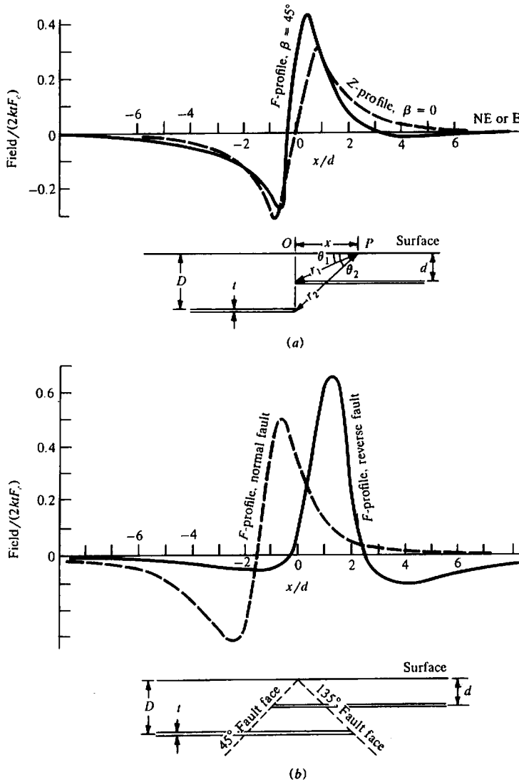
Figure 3.23. Thin-sheet fault approximation; D = 2d , t = 60^\circ . (a) F, Z profiles for vertical faults striking N-S and SE-NW ( \beta = 0^\circ, 45^\circ ). (b) F profiles for normal and reverse faults striking E-W; fault dip 45^\circ, 135^\circ .
