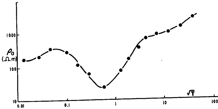
Figure 6.23. Magnetotelluric sounding over multiple beds.
