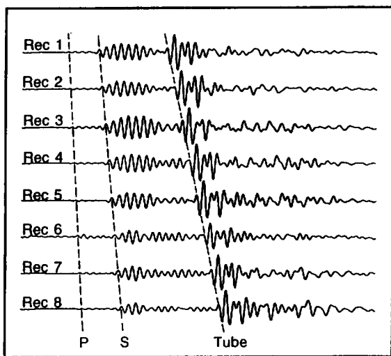
Figure 11.21. Waveforms recorded in a borehole. (a) Waveform showing formation arrivals ( P and S waves), mud arrivals, and boundary (tube-wave) arrivals. (Courtesy Schlumberger.) (b) Waveforms from eight broad-band receivers spaced at intervals of 6 in. (15 cm). (After Morris, Little, and Letton, 1984.)
