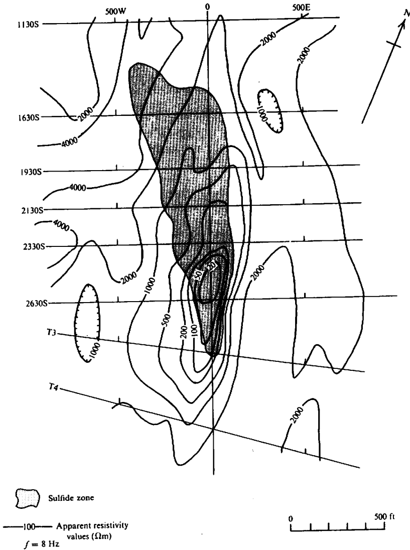
Figure 6.26. Telluric data from 8 Hz survey over massive sulfides, New Brunswick.
