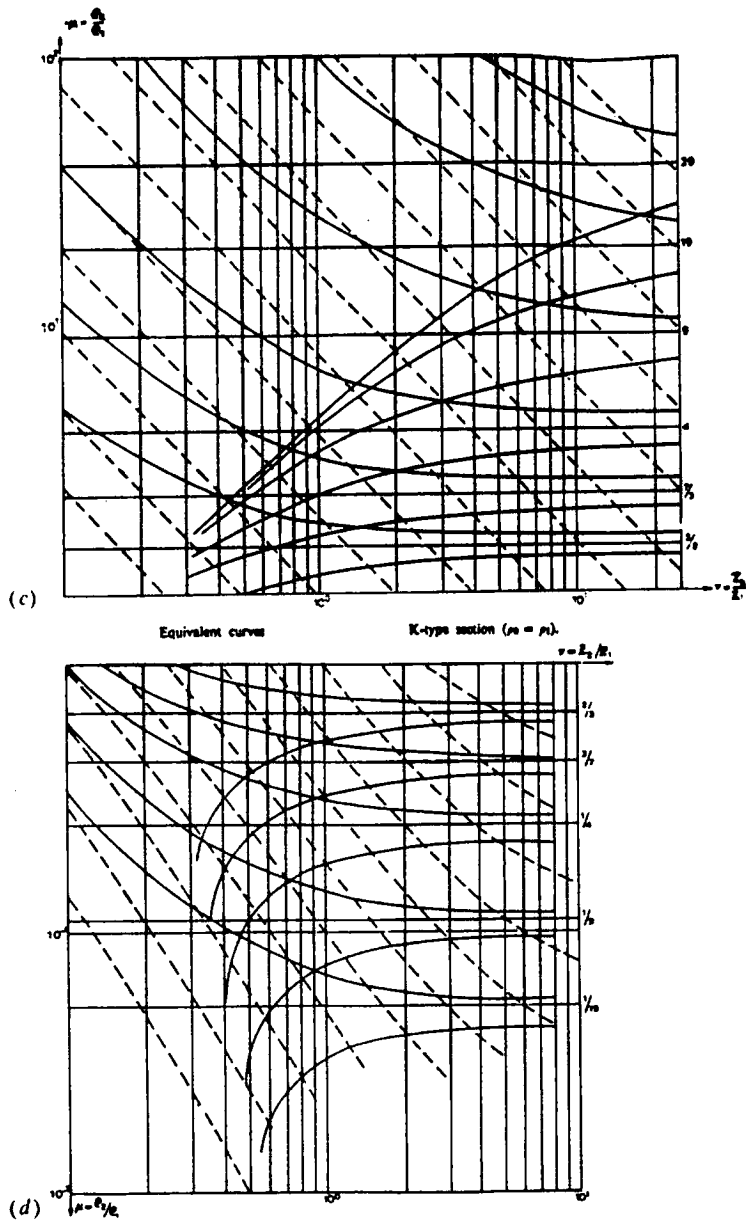
Figure 8.32. (Continued) (c) K-type section, \rho_3 = \rho_1 . (d) Q-type section \rho_3 = 0 .
