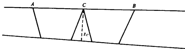
Figure 4.95. Refraction profile for determining depth to bedrock.
