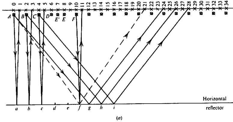
Figure 4.45. Symmetrical spread with continuous subsurface coverage.
