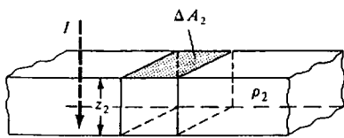
Figure 8.30. Effect of topography on expanding Wenner spread.
