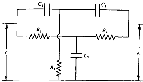
Figure 7.13. Twin-T network for EM receivers. \omega^2 = 1/(2C_1^2R_1R_2) = 2/(C_1C_2R_1^2) . Generally R_2 \approx 2R_1 , C_2 \approx 2C_1 for convenience in design.
