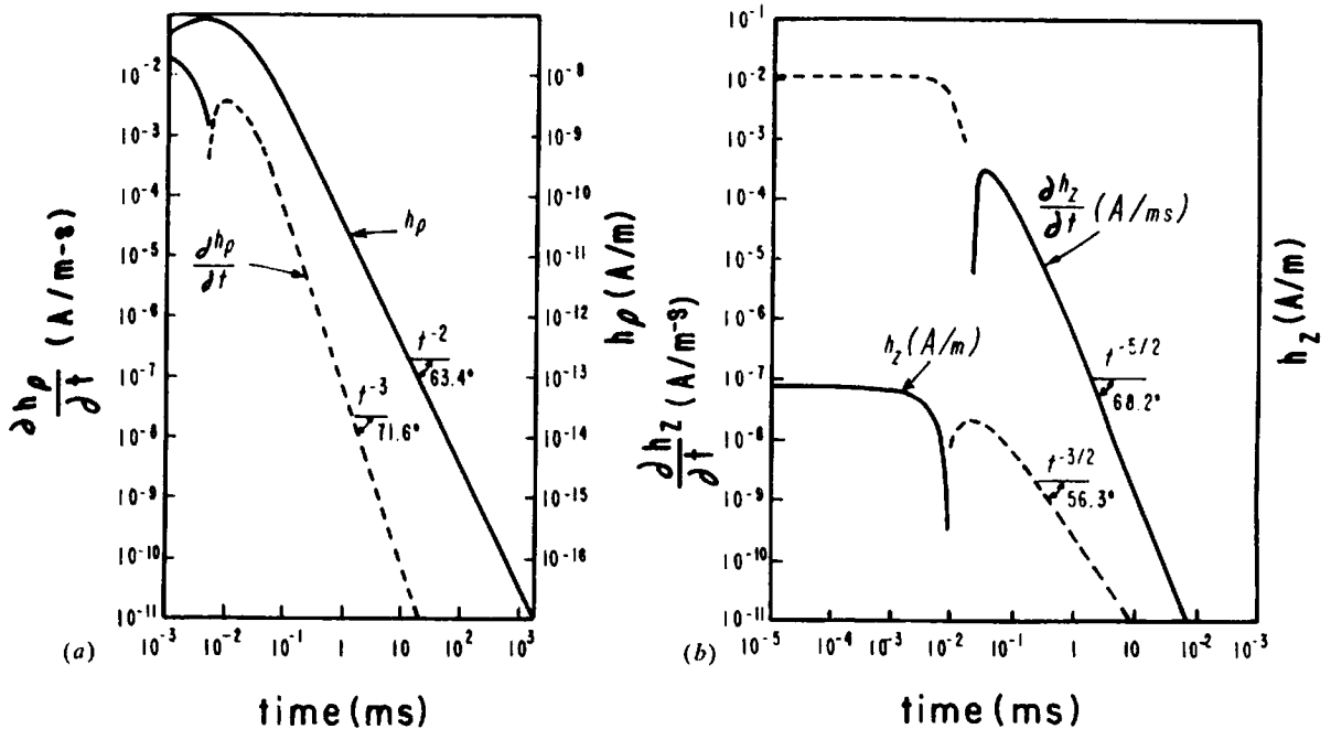
Figure 7.12. TD transient decay curves at a point 100 m from a vertical magnetic dipole on 100 \Omega\text{m} homogeneous earth. (From Ward and Hohmann, 1988.) (a) h_p and \partial h_p/\partial t . (b) h_z and \partial h_z/\partial t .
