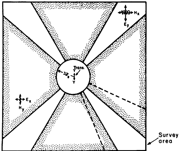
Figure 6.17. AMT survey with dipole source. Shaded areas represent areas with minimum coupling between Y-oriented transmitter (center) and E_x - H_y receiver orientation; dotted lines show approximate limits of strong coupling for E_y - H_x receiver directions. (After Goldstein and Strangway, 1975.)
