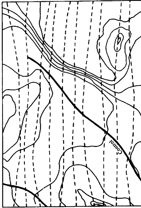
--- Flight lines — Control lines ~ Total field contours (c)
