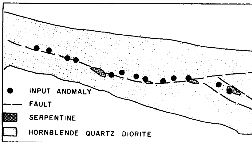
Figure 7.91. Structural mapping with Input system; Lake Wanipigow area, Southeastern Manitoba. (After Dyck, Becker, and Collett, 1975.)
