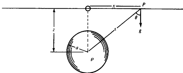
Figure 2.23. Gravity effect of a sphere.
