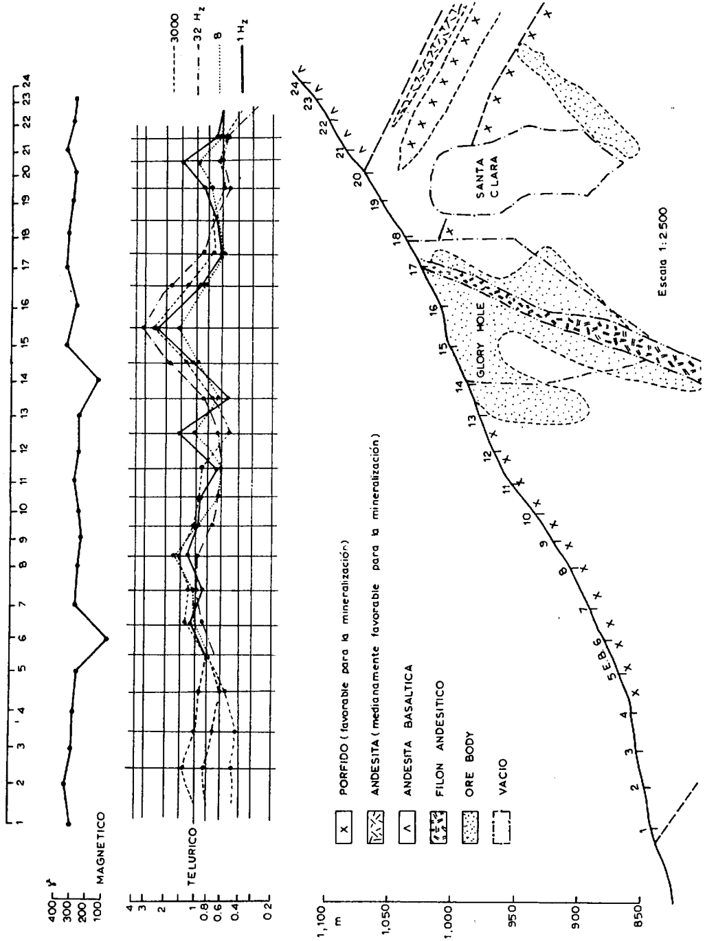
Figure 6.39. Geologic section with magnetic and telluric surface profiles over mine area, Chile.
