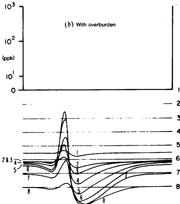
Figure 7.52. Approximate effect of conductive overburden. \ell = d = 600 m, z = 50 m, T-R = 100 m, \sigma = 30 S, \text{dip} = 30^\circ . Channel numbers are at the right in (a) and (b), channel response at the left. (After Bartel and Hohmann, 1985). (a) Response without overburden. (b) Response with overburden. (c) Overburden model.
