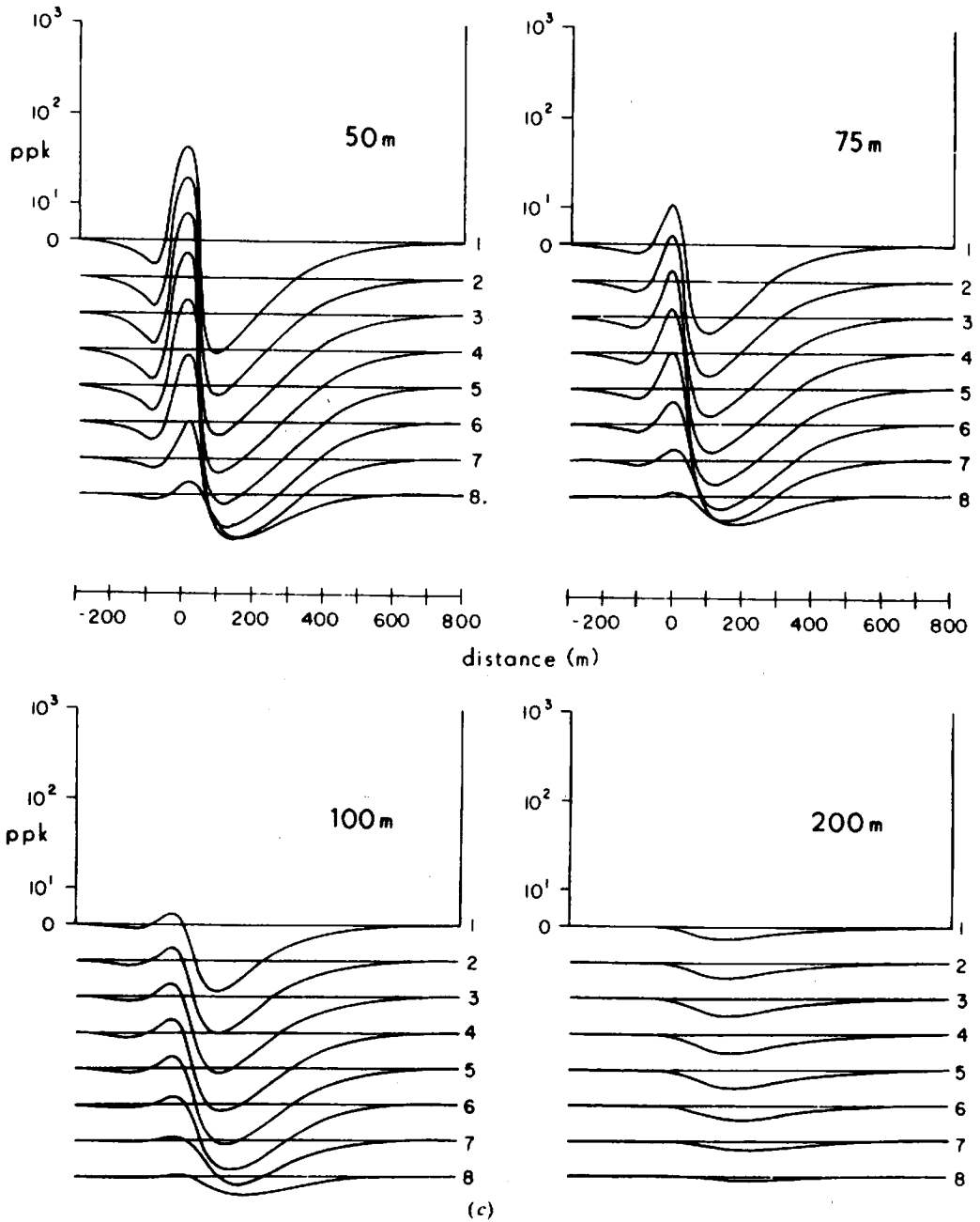
Figure 7.50. (Continued) (c) Same as (b) except dip = 30°.
