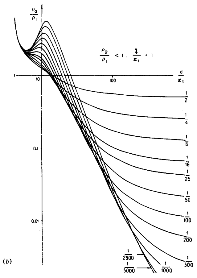
Figure 7.76. Master curves of late-time (\rho_0/\rho_1) versus (d/z_1) . [Parts (a) and (b): After McNeill, 1980; parts (c) to (f): After Kaufmann and Keller, 1983.] (a) Two-layer curves for resistive basement. (b) Same as (a) except for conductive basement.
