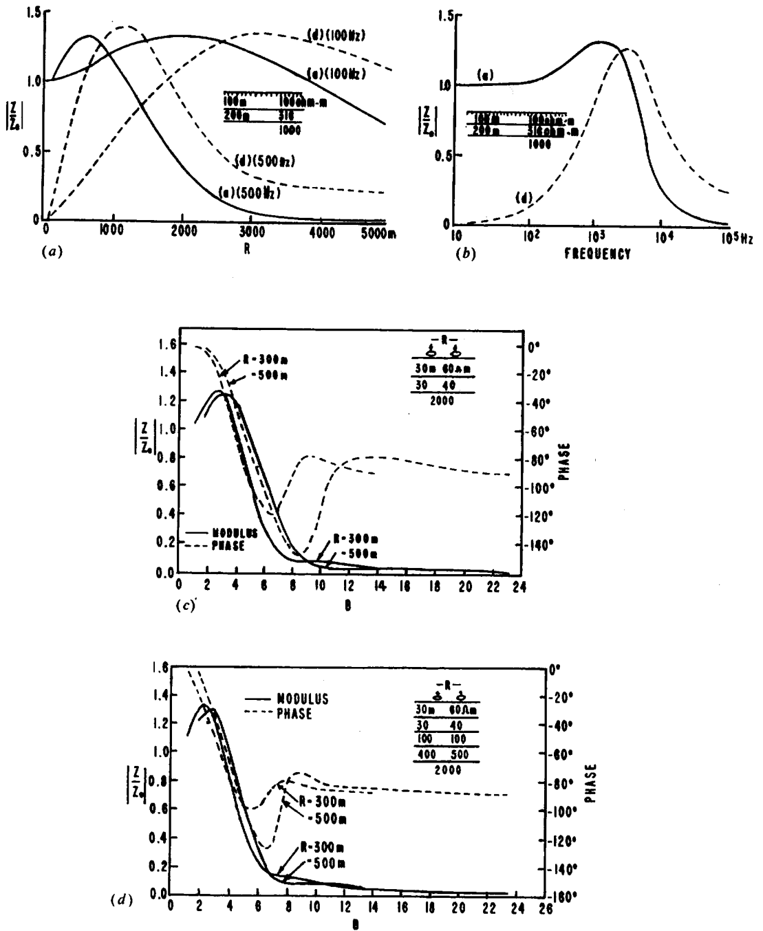
Figure 7.74. Mutual coupling ratio (modulus and phase) for systems (a) and (d) of Equation (7.41) over multilayer earth. (After Patra and Mallick, 1980.) (a) Modulus and phase for systems (a) and (d) over three-layer type-A earth (§8.6.4b), geometric sounding. (b) As in (a) except parametric sounding. (c) Modulus and phase as functions of B for a three-layer type-H earth, system (a). (d) As in (c) except for a five-layer earth.
