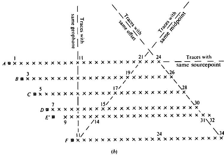
Figure 4.46. Common-midpoint profiles. The symbols x and O represent geophone groups and sourcepoints, respectively. (a) Vertical section illustrating common-midpoint profiling. (b) Stacking chart.
