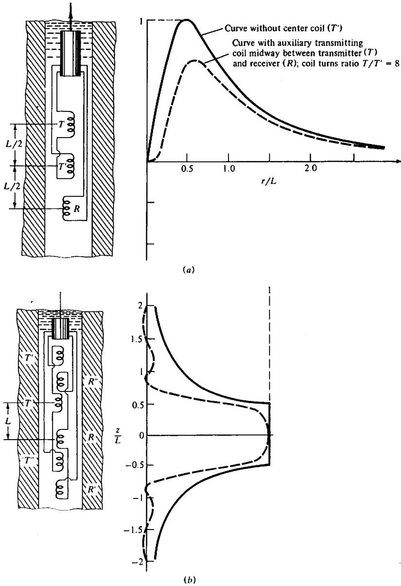
Figure 11.8. Geometric factors for induction sondes without (solid curves) and with (dashed curves) auxiliary coils (T', T'', R', R''). (After Doll, 1949.) (a) Radial factor g(r) . (b) Depth factor g(z) .
