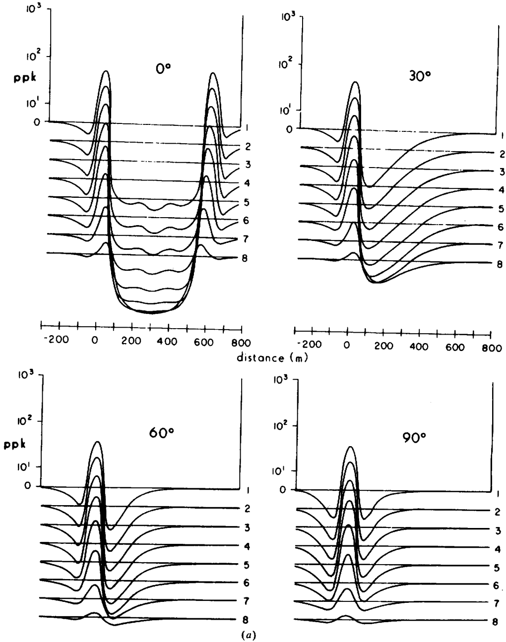
Figure 7.50. PEM(1) response to a dipping sheet as a function of dip, depth, and TCP. \ell = d = 600 m, T-R = 100 m, TCP = \alpha t = 30 S [except in (d)]. (After Bartel and Hohmann, 1985.) (a) Effect of dip; z = 50 m.
