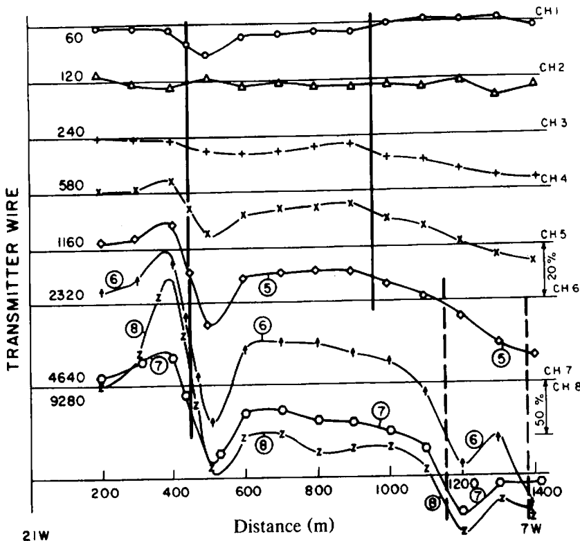
Figure 7.117. Profiles of seven-channel UTEM TD response, test site, Ontario.
